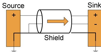
Figure 4 - 3-Wire Unbalanced Source to Balanced Sink Connection
