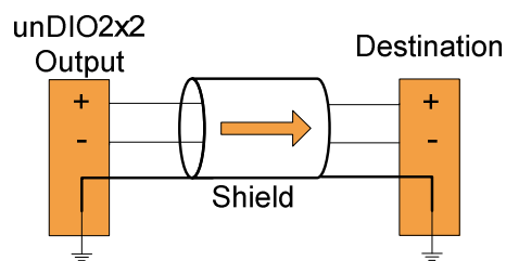
Figure 5 - Output to Balanced Destination Connection
