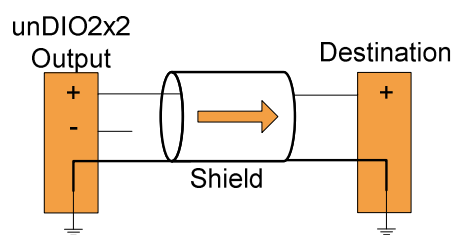
Figure 6 - Output to Unbalanced Destination
